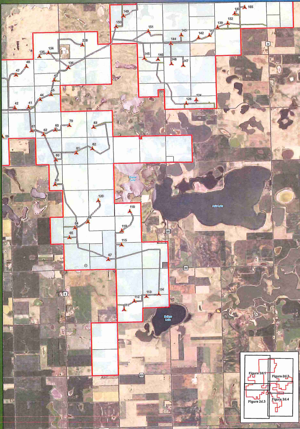
Figure 2d.4 Preliminary Project Layout Map Series Vestas V110
