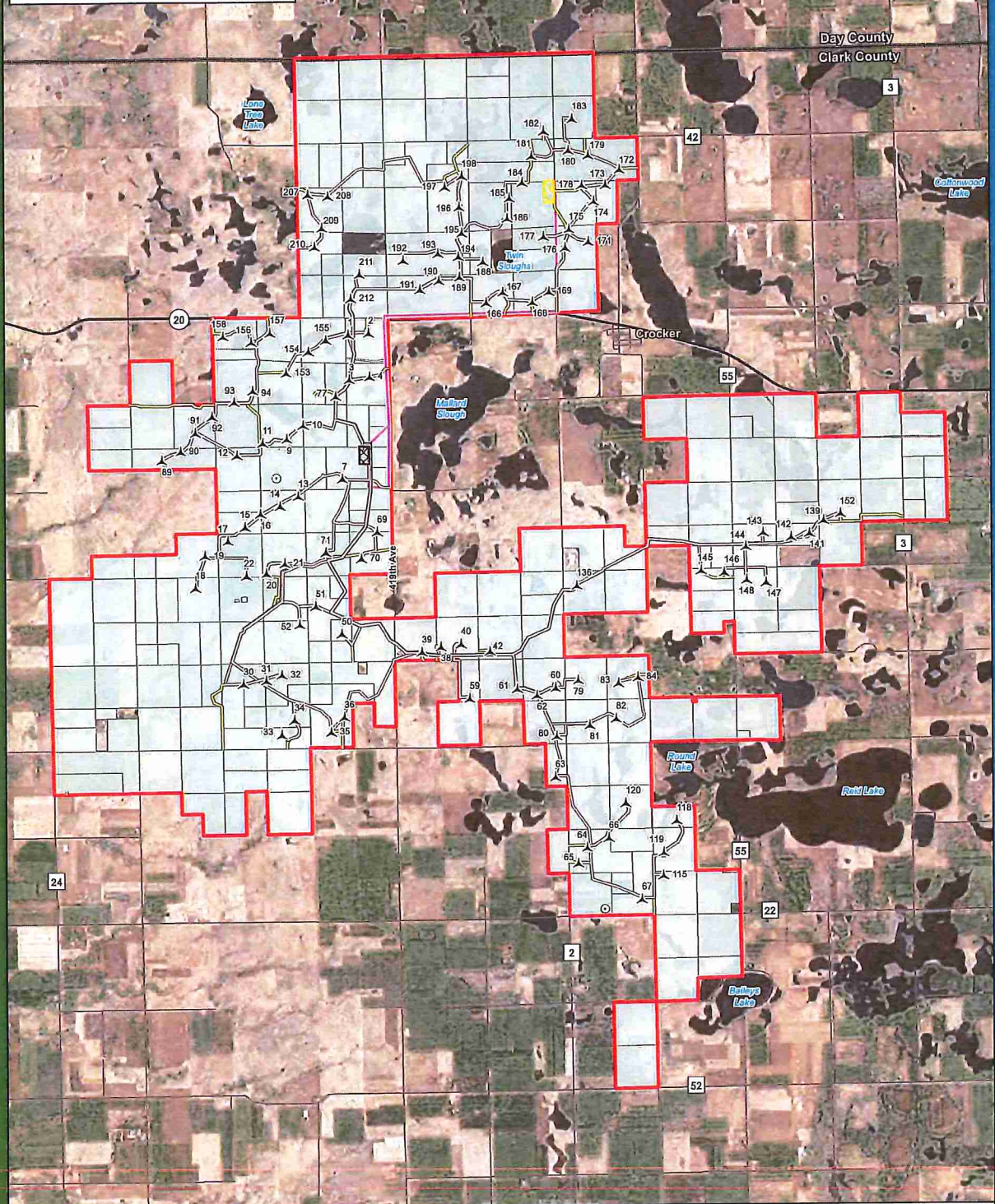
Figure 2b Preliminary Project Layout Vestas V136
