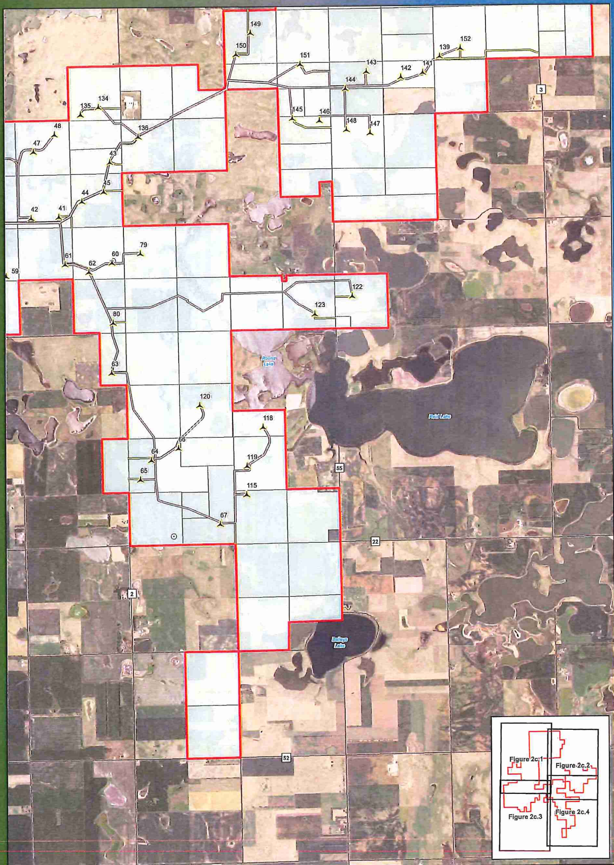
Figure 2c.4 Preliminary Project Layout Map Series GE 2.5-116
