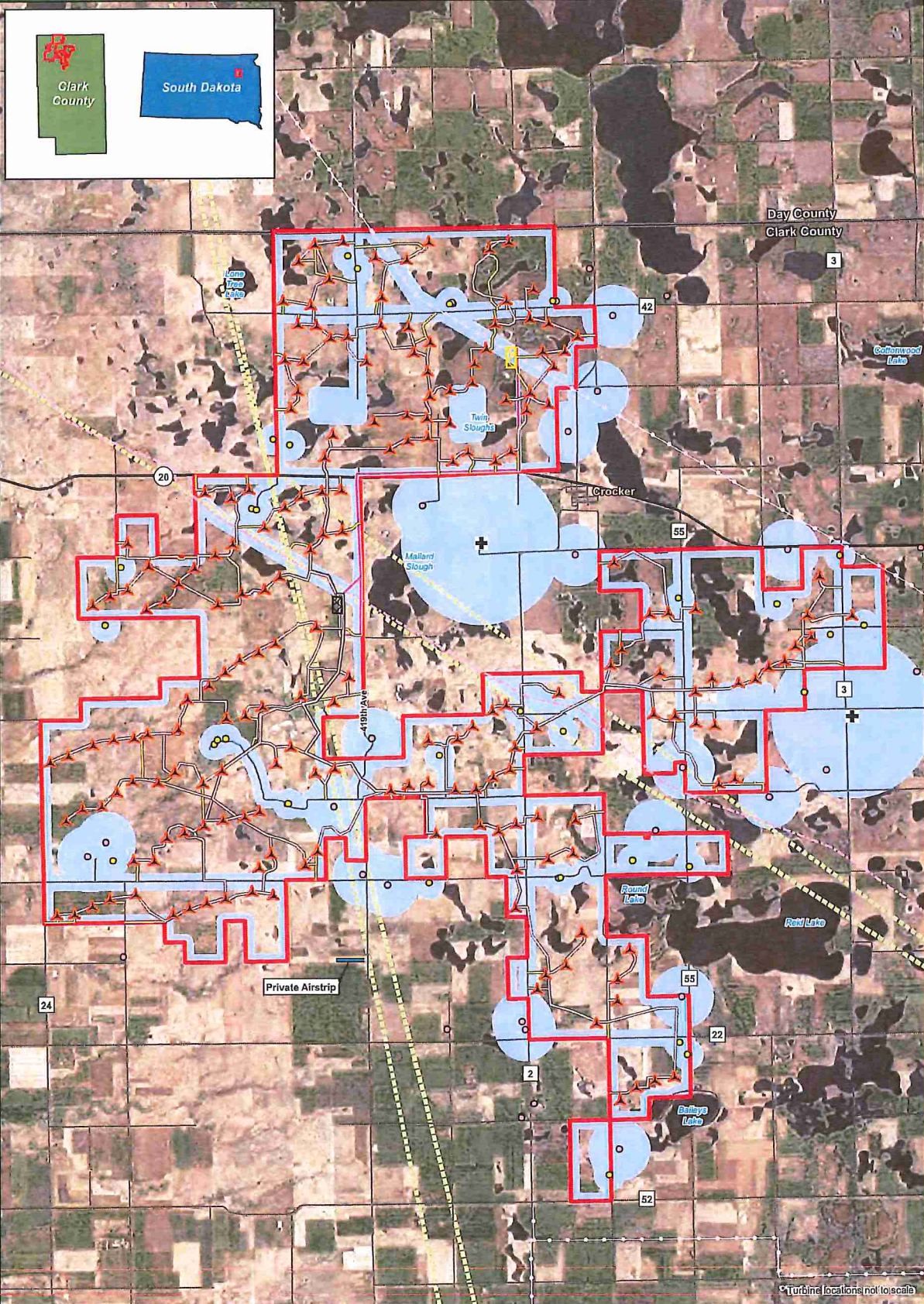
Figure 10d Project Layout and Constraints Vestas V110
