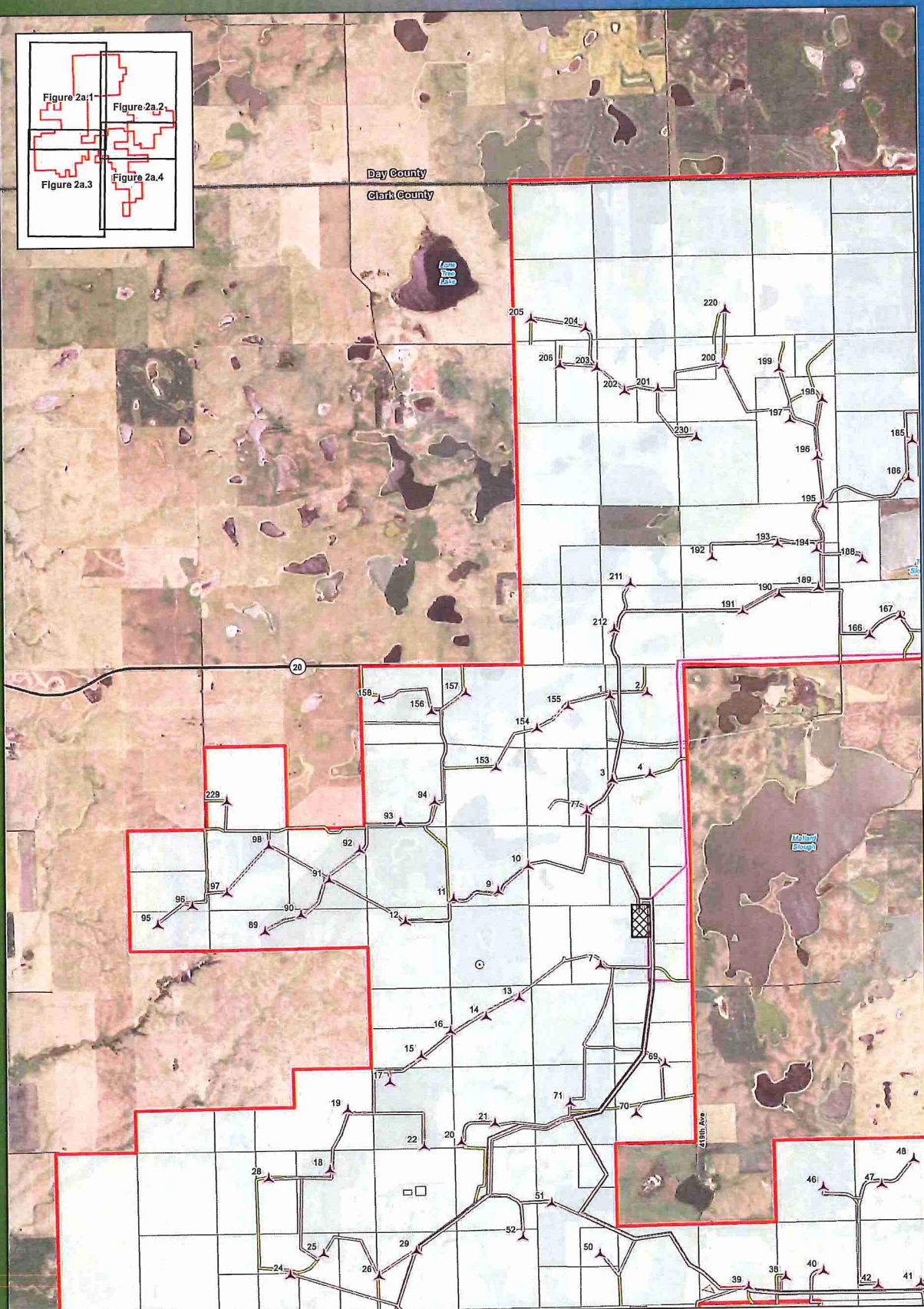
Figure 2a.1 Preliminary Project Layout Map Series Gamesa G126
