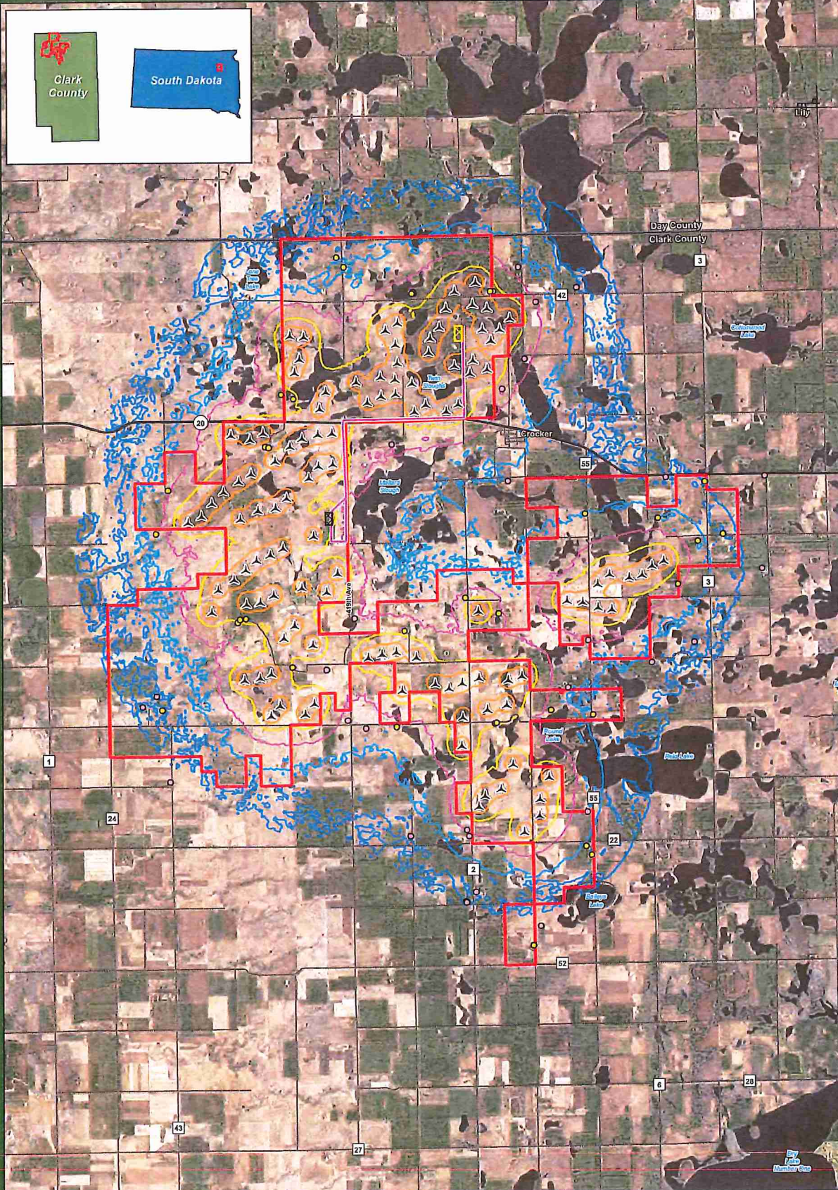
Figure 8b Sound/Noise Vestas V136 Crocker Wind Farm Clark County, SD 45.079602, -97.845696
