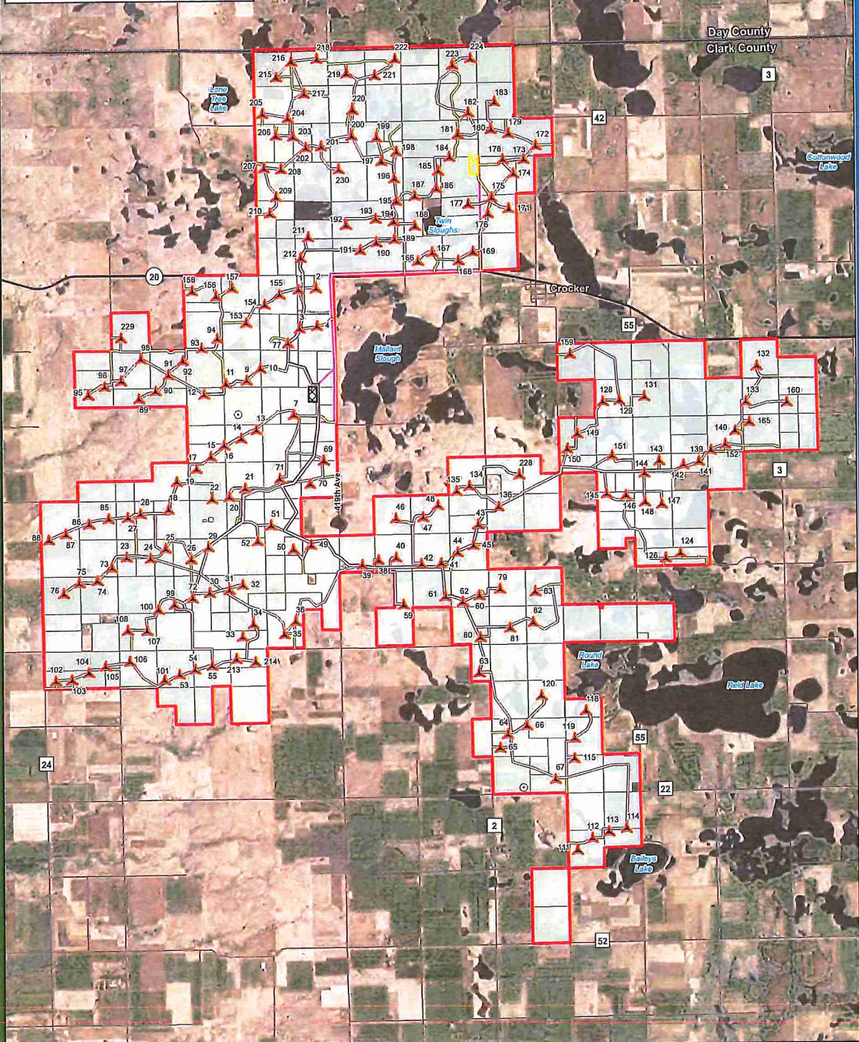
Figure 2d Preliminary Project Layout Vestas V110
